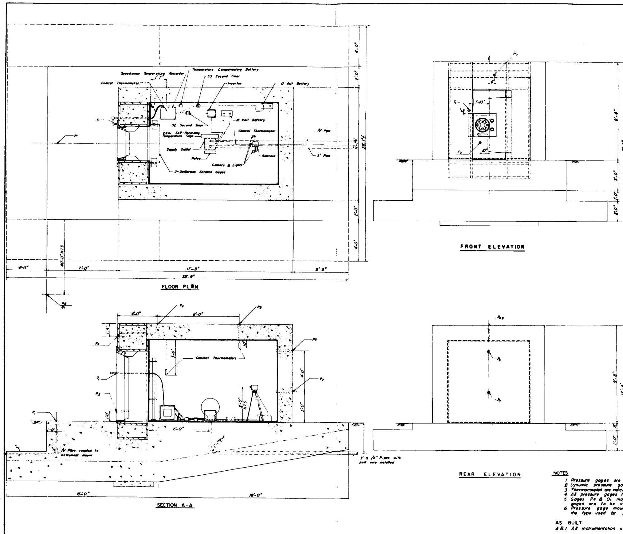
Fig. 7—Instrumentation of structure 30.4.
